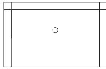
TV Back Panel 1623001 (for Fridge Chest) D0.75xW57xH36 1623002 (for 40" TV Chest) D0.75xW39xH36
