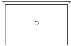
TV Back Panel 1923001 (for Fridge Chest) D1.25xW57xH36 1923002 (for 40" TV Chest) D1.25xW39xH36
